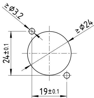
Panel Cut out dimension
