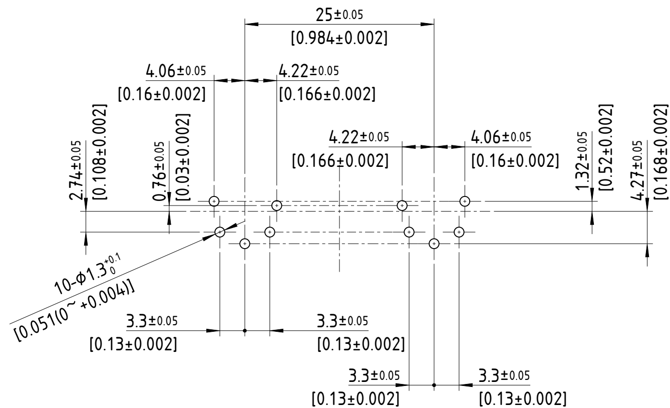
PCB cut out dimension (rear side):
