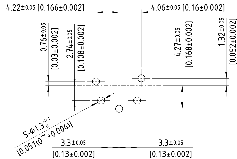
PCB cut out dimension (rear side):
