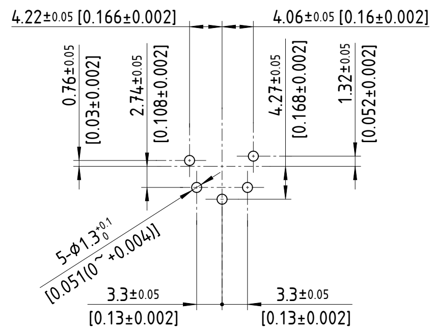
PCB cut out dimension (rear side):
