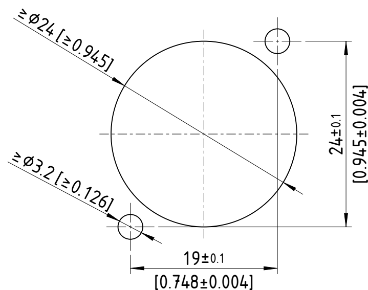
Panel cut out dimension (rear side):
