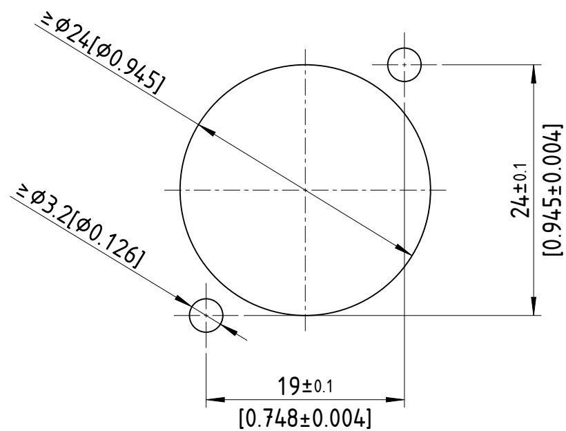
Panel cut out dimension (rear side):
