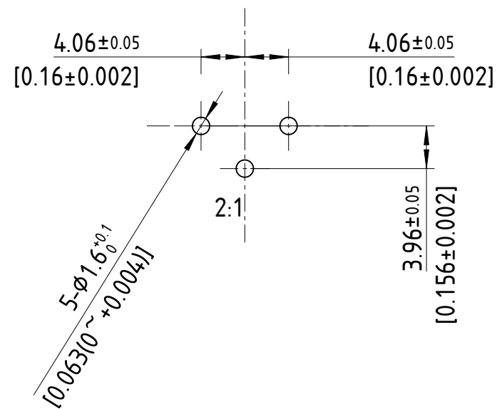
PCB cut out dimension (rear side):
