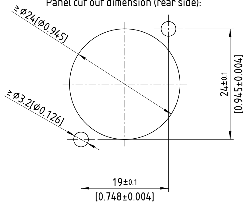
Panel cut out dimension (rear side):
