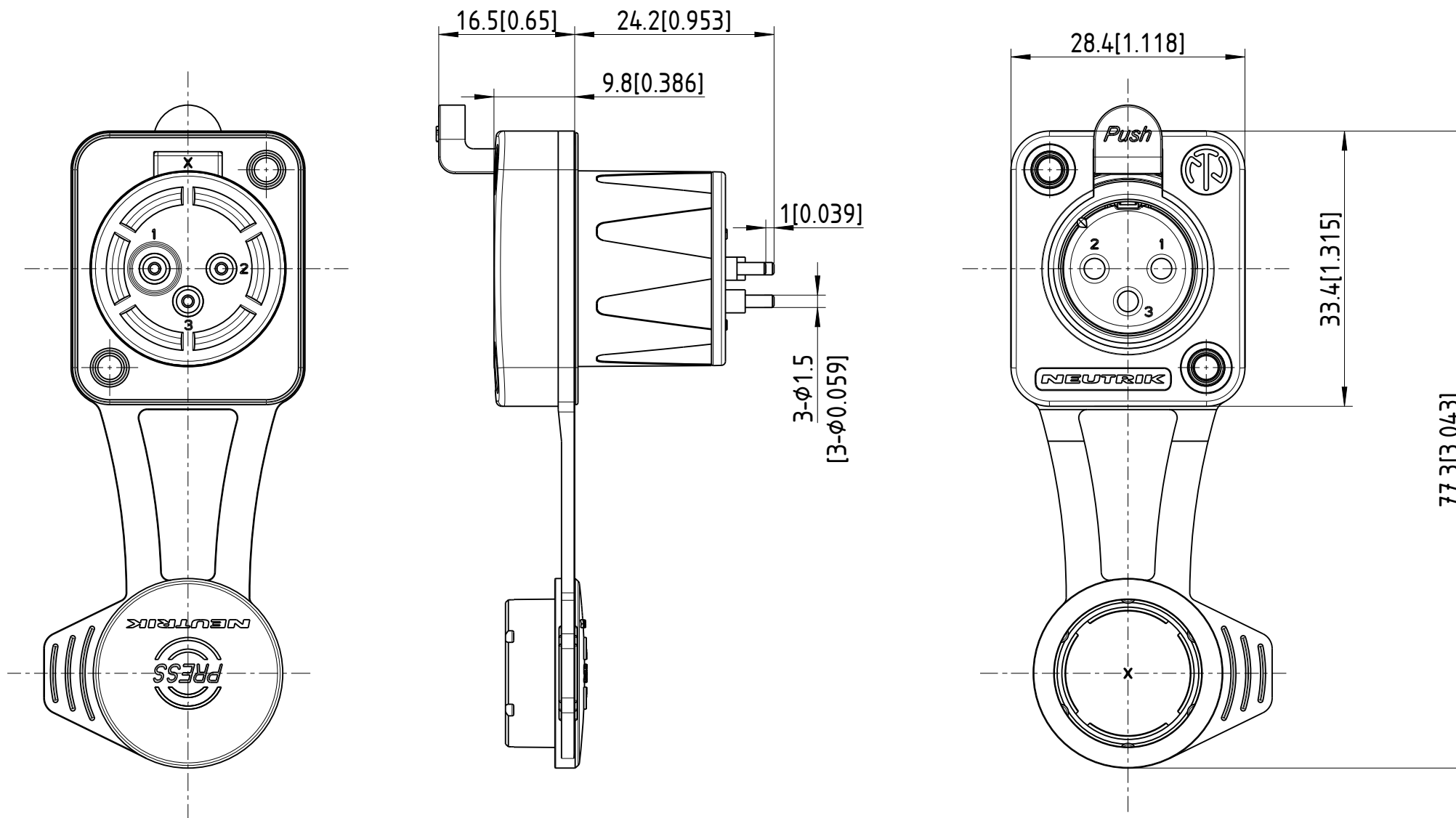
PCB cut out dimension (rear side):
